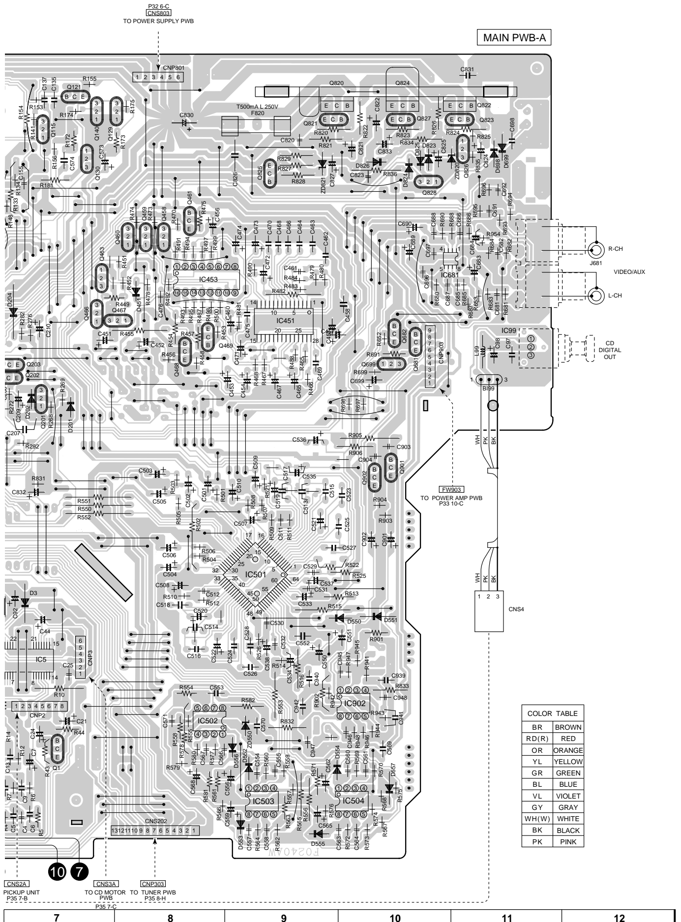
Figure 3 WIRING SIDE OF P.W.BOARD (1/2)
